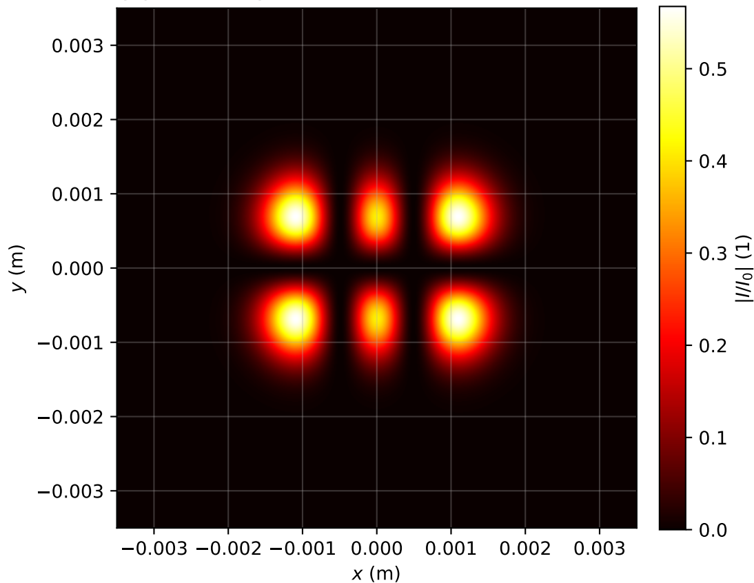
Intensity profile I(x, y, z = 1.911)/I_0 , P_{in}=0.5P_{cr} , artificial time
